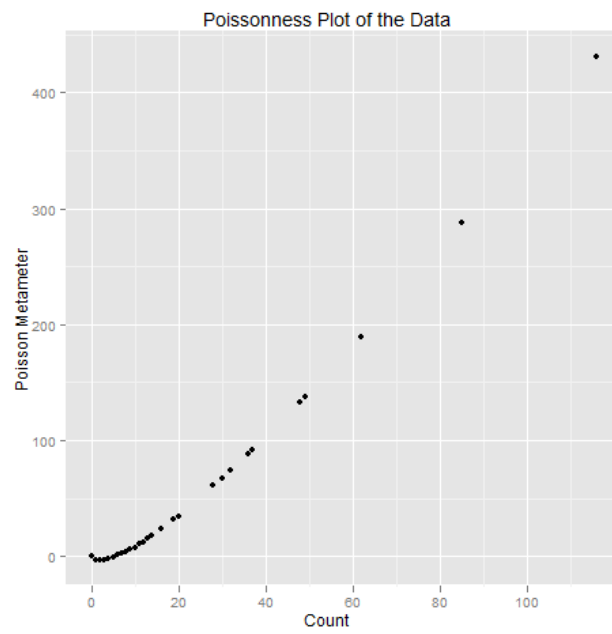
SFigure 2. Poissonness plot for 10 year interval.
