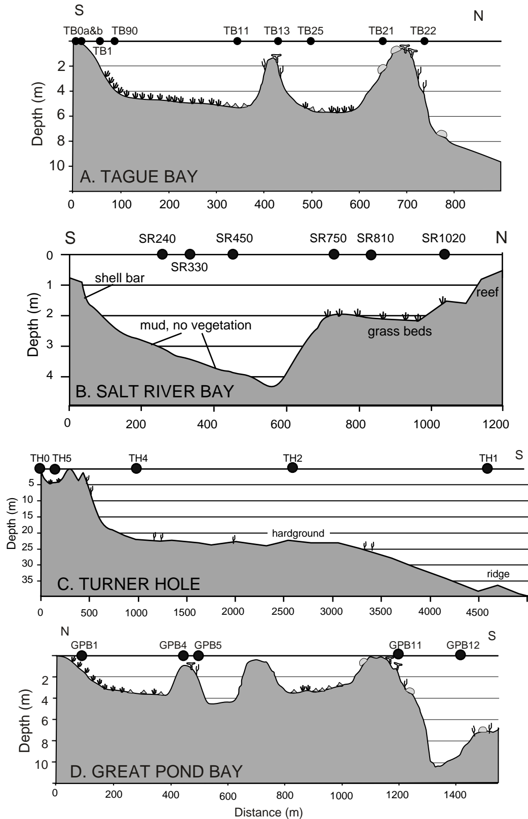
Archived figure. Depth and bottom type profiles across each reef-lagoon system. Note that vertical and horizontal scales change, as does north-south orientation (so that all can be displayed onshore to offshore).
