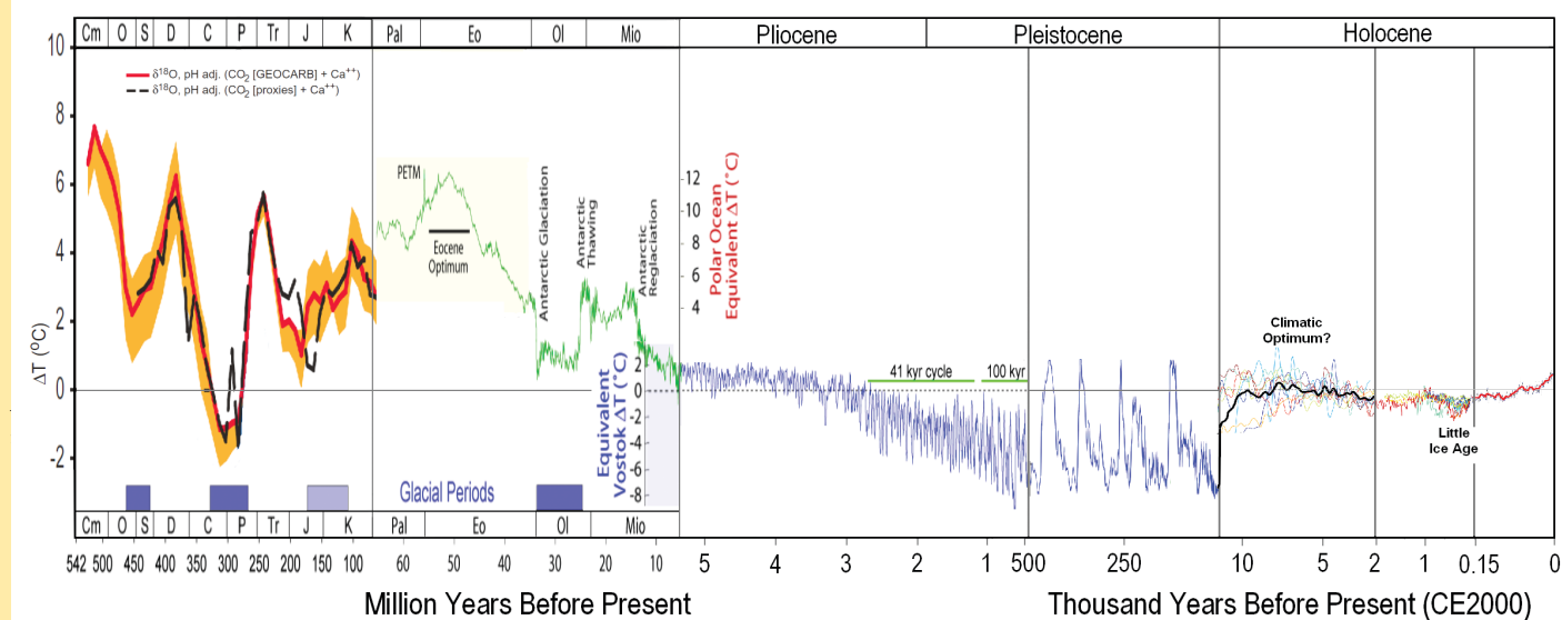
Figure 2: Schematic of paleotemperatures for the Phanerozoic. http://en.wikipedia.org/wiki/File:All_palaeotemps.png , accessed 21 May 2013. Compiled from multiple sources (information on website). As the methods used to determine temperature are not identical, the variations should be taken as relative and not absolute. However, the figure represents current thinking about relative temperature changes.
