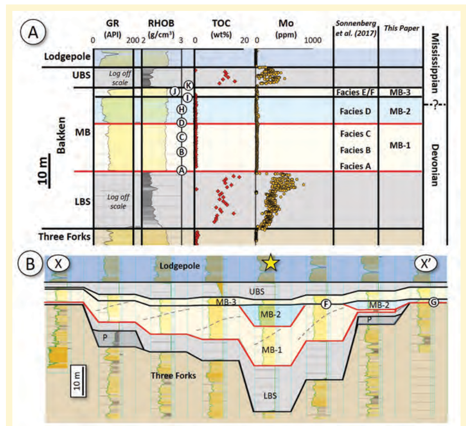
Figure 2: A) Type log for the Bakken in North Dakota showing stratigraphic units defined in the text and relationship between our stratigraphic terminology and that of Sonnenberg et al. (2017). B) Interpreted east-west gamma-ray log cross section through the Williston Basin (location in Figure 1C). All wells on the section are cored through the entire Bakken, enabling confident assignment of facies and surface picks. Yellow star in Part B shows location of Type Log shown in 2A. Lettered circles (A-K) show location of photos in Figure 3.
