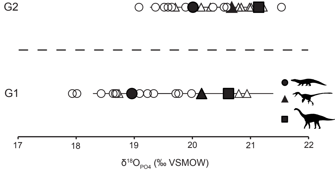
Supplementary Data 2. \delta^{18}\text{O}_{\text{PO}_4} values for crocodilians (=circles), theropods (=triangles) and sauropods (=squares) in levels G1 and G2. Mean values are given in larger solid symbols.
